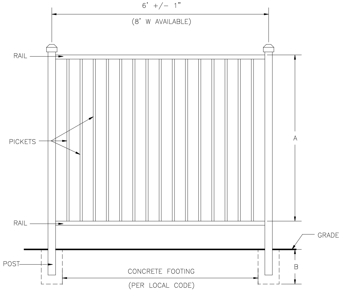
UAF 200 FLAT TOP - 2-RAIL FLUSH
