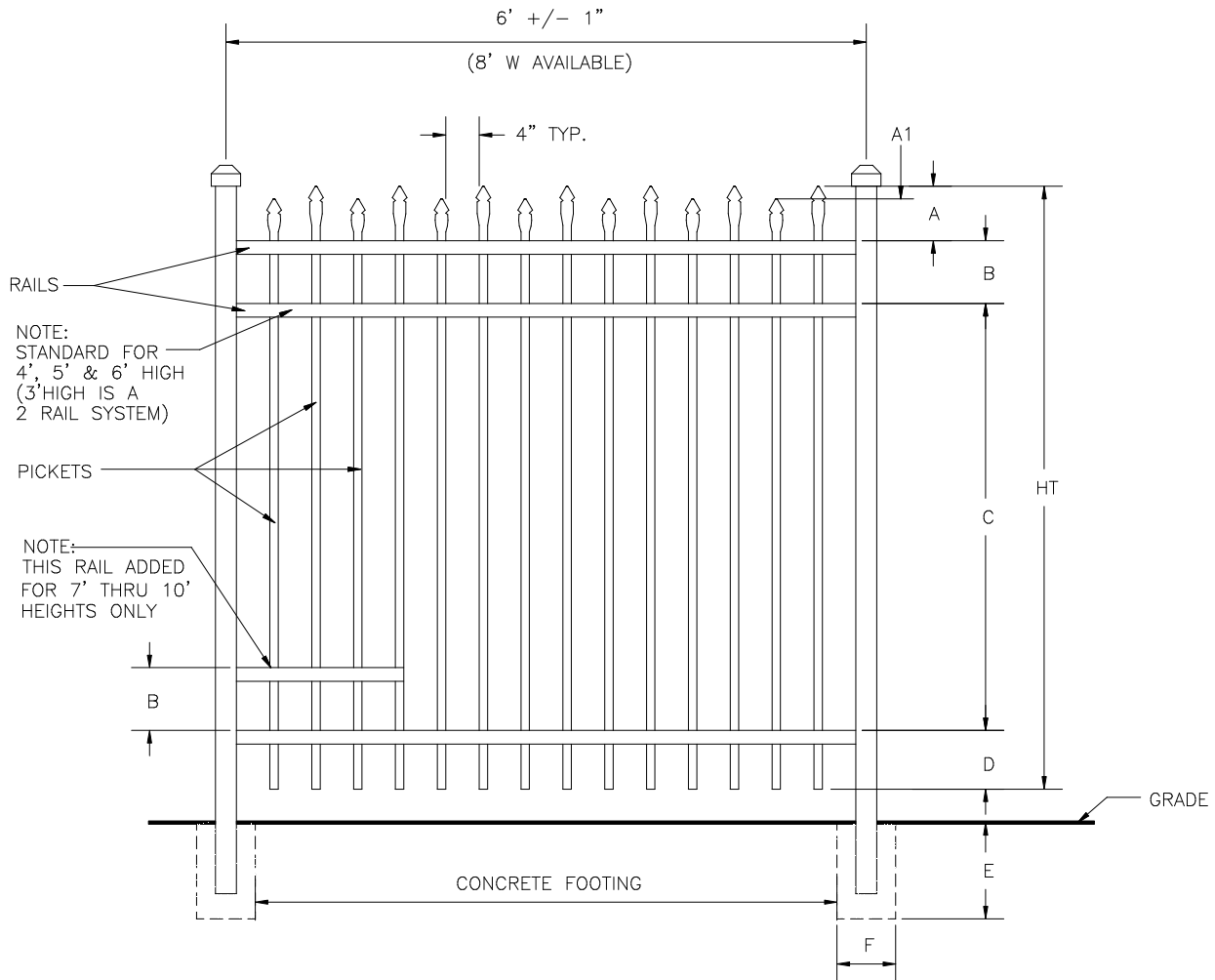
UAS 150 STAGGERED SPEAR TOP
