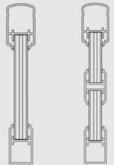
Ultra™ Vinyl Privacy 2-Rail System Ultra™ Vinyl Privacy 3-Rail System
