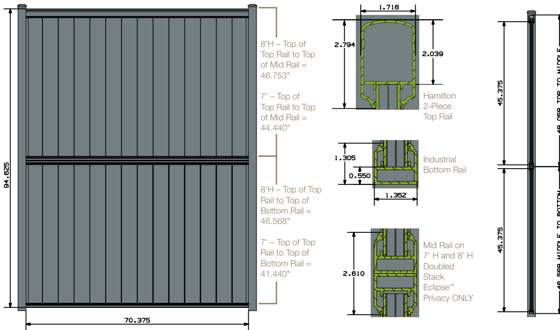
ECLIPSE™ PRIVACY PANEL 3-RAIL DOUBLE STACK STANDARDS
