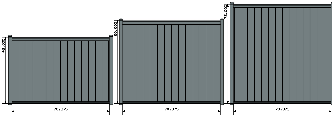
ECLIPSE™ PRIVACY PANEL 2-RAIL STANDARDS
