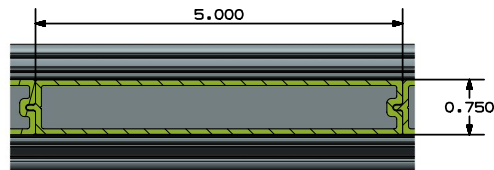
ECLIPSE™ PRIVACY TONGUE AND GROOVE BOARD SECTION
