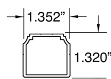
Bottom Rail
