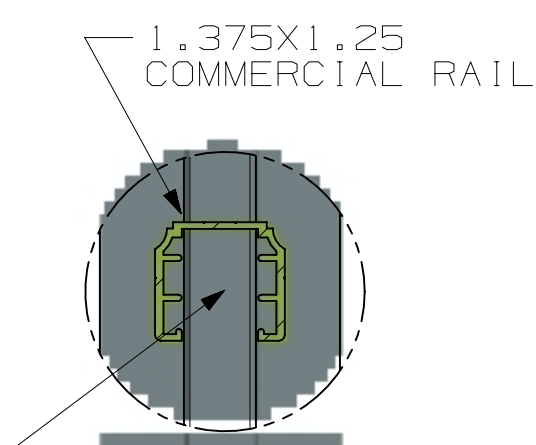
DETAIL D SCALE 1:4
