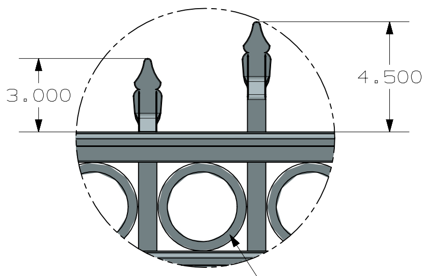
DETAIL D SCALE 1:4
