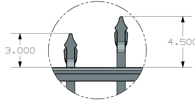
DETAIL D SCALE 1:4
